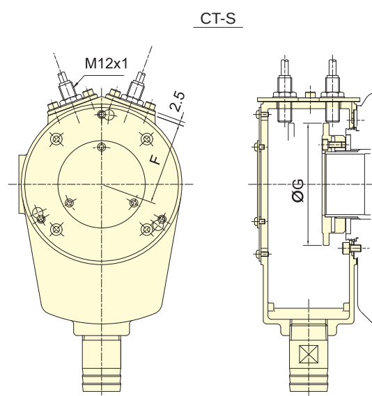
Coolant Collector with Detecting Ring
