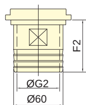
Ø60 Drain port Only use to CT-S08B/CT-S10B/CT-S12B
