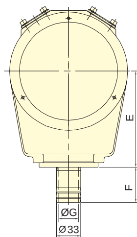
Coolant Collector
