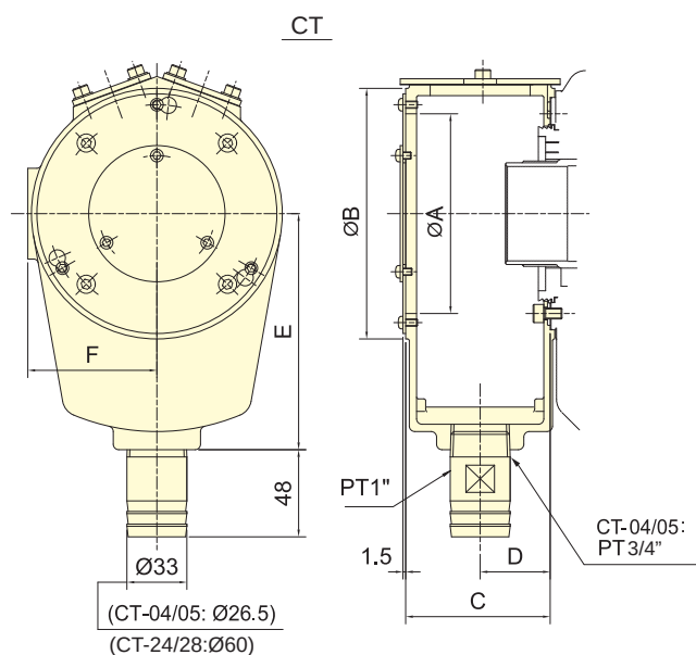
Coolant Collector
