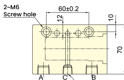
RC1/4" Airtight detection port
