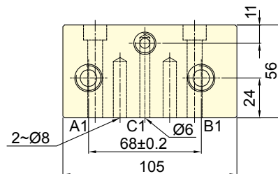
RC1/4" Airtight detection port
