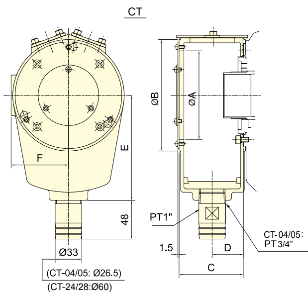
Coolant Collector
