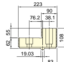
Hardened jaw HJ-50 for V-40"-79"
