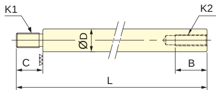
中實拉桿詳圖 Detail of Draw Bar L = A - G1_{max} - G2_{min} - 4 + C
