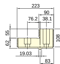
硬爪 HJ-50 for V-40"-79" Hardened jaw
