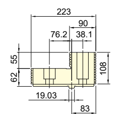
硬爪 HJ-50 for V-40"~79"
