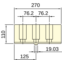
Soft jaw SJ-50 for V-40"-50" SJ-63 for V-63"-79"
