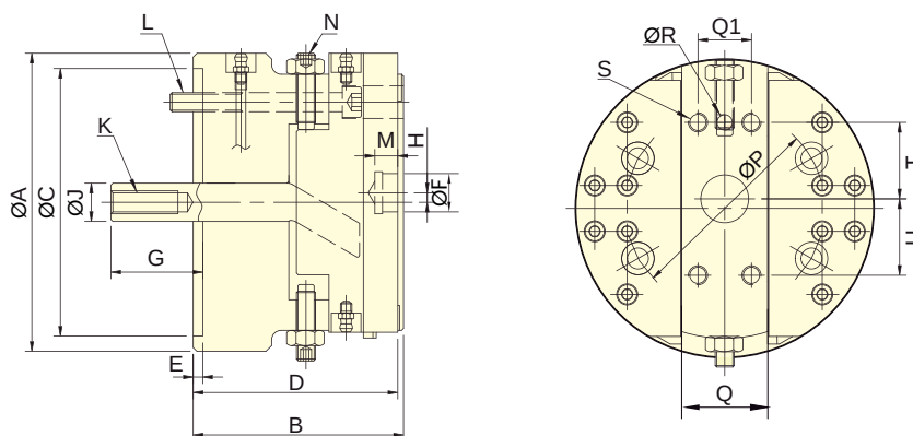
WEDGE PLUNGER FA-610 FA-812
