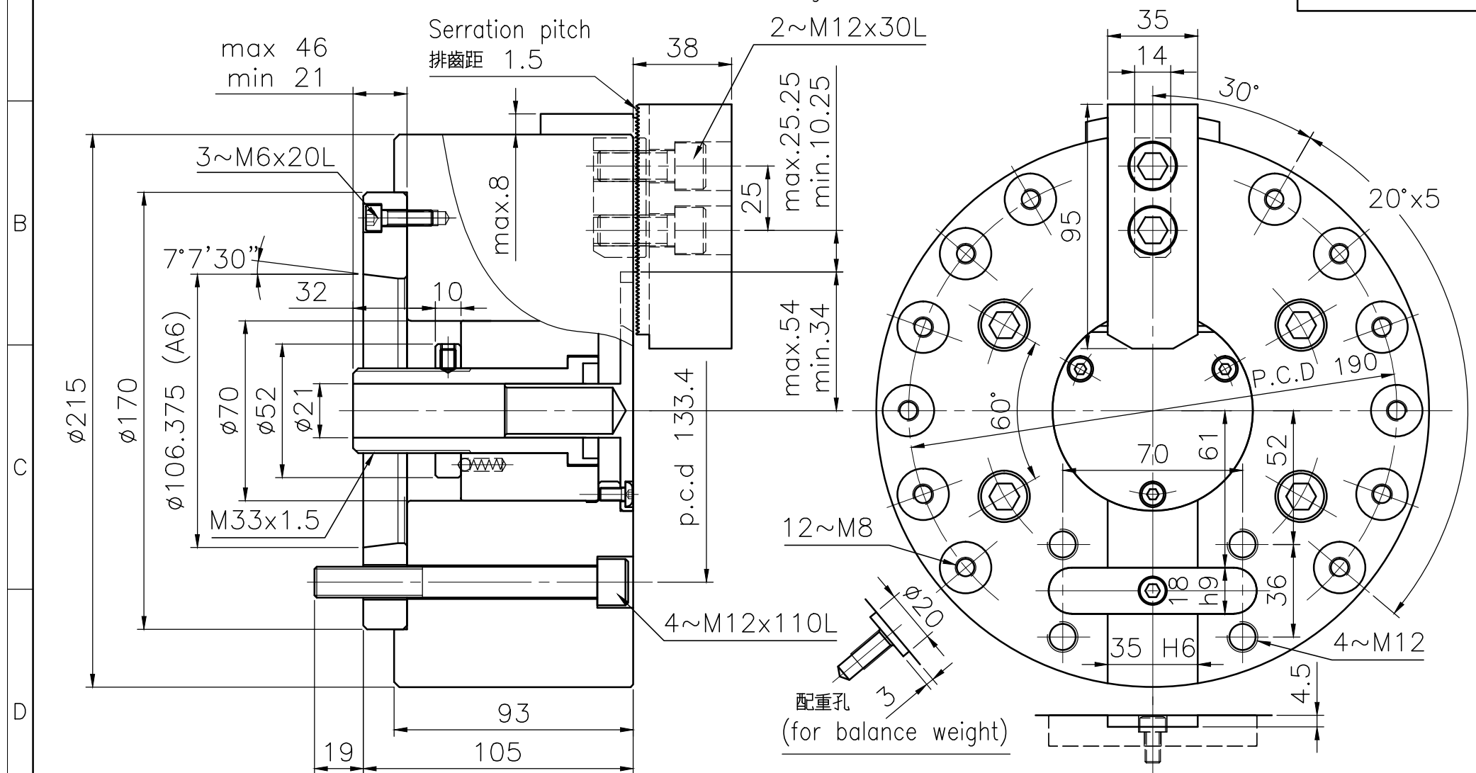
單爪中實長行程夾頭 Extra long jaw stroke single-jaw power chuck
