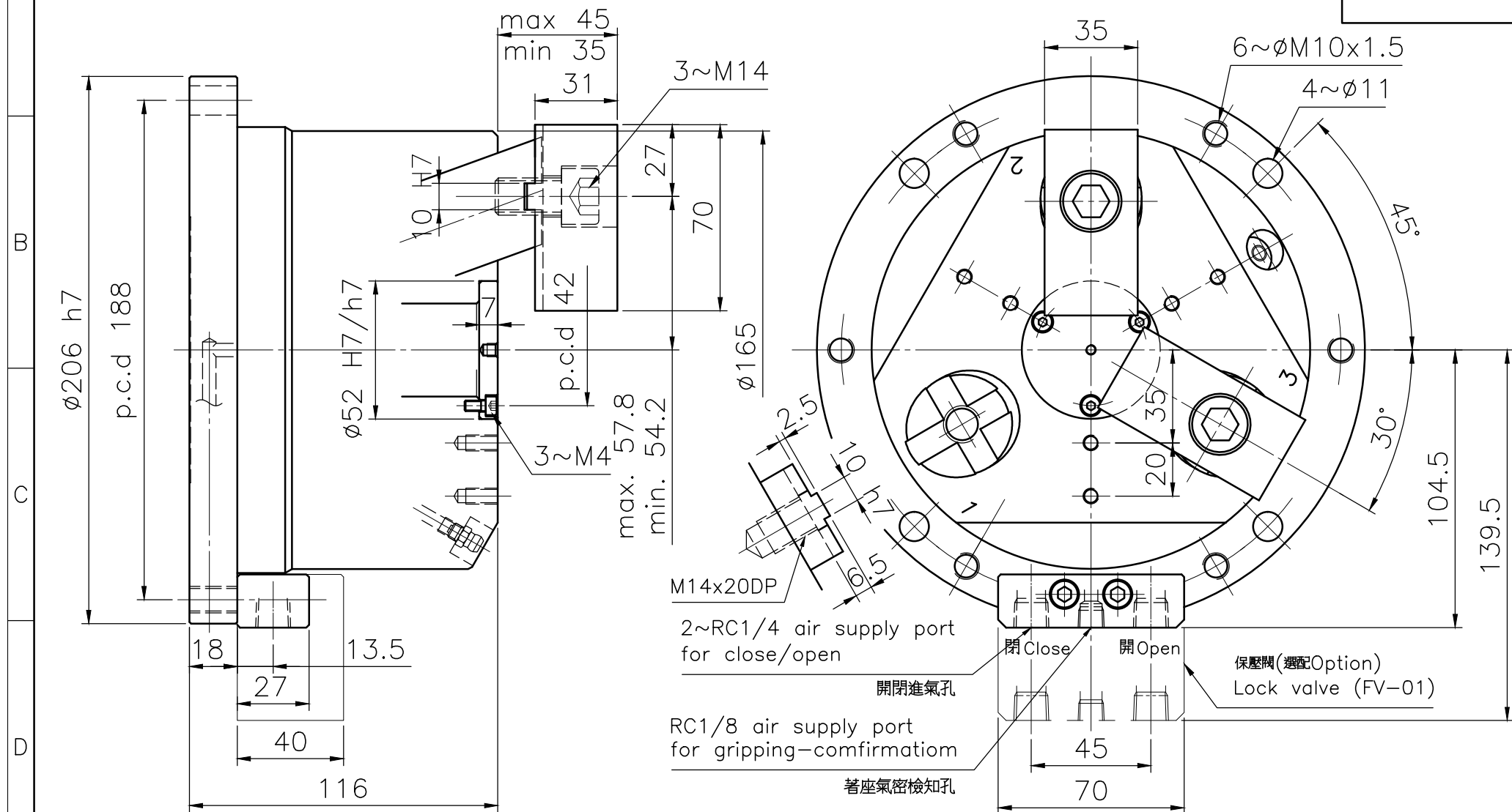
立置式後拉三爪夾頭 Stationary Pull Back Chuck
