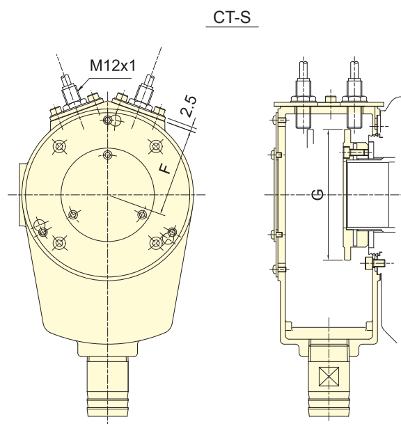
Coolant Collector with Detecting Ring
