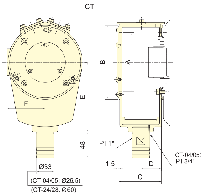
Coolant Collector
