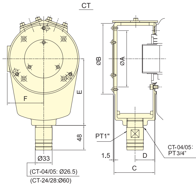
Coolant Collector
