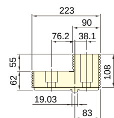
Hardened jaw HJ-50 for V-40"~79"
